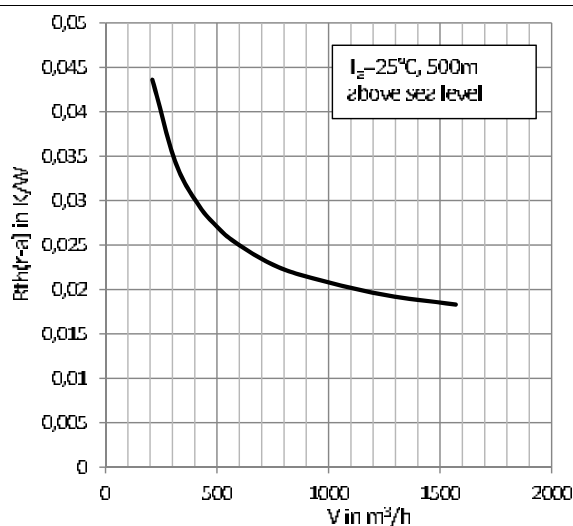
Fig. 9: Thermal resistance R_{\text{th}}(r-a) versus flow rate V
