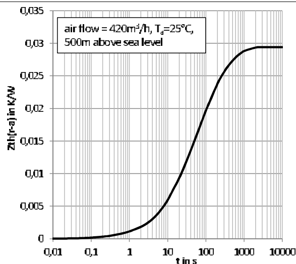
Fig. 7: Transient thermal impedance Z_{\text{th}}(r-a)
