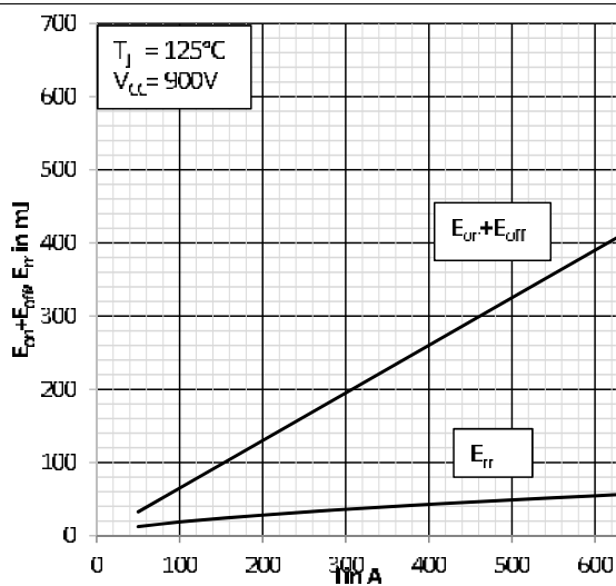
Fig. 3: Typical energy losses E = f(I_C, V_{CE})
